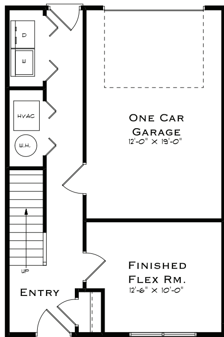
FIRST FLOOR PLAN WITH GARAGE
